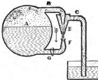
FIG. 186.—Diagram Illustrating the Operation of a Boiler-Feeding Injector. A is the boiler; B , a pipe leading steam to the nozzle of the injector; C , a pipe leading from the feed tank; E , the nozzle, through which the steam forces the water raised; F , the feed pipe leading to the boiler; G , a control cock.
